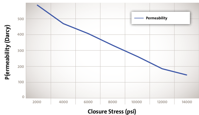
UltraProp® Sintered Bauxite Permeability (@300°F, 2 lbs/ft 2 )
